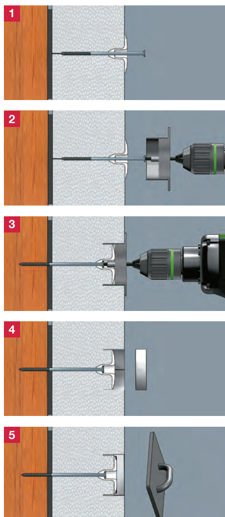
Countersunk installation acc. to the EJOT STR principle with ejothem STR cap
