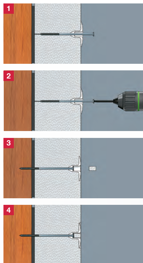
Surface fix installation with ejothem STR plug
