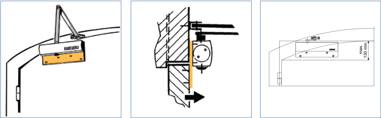
TS 2000 V door leaf installation/hinge side segmental arch
