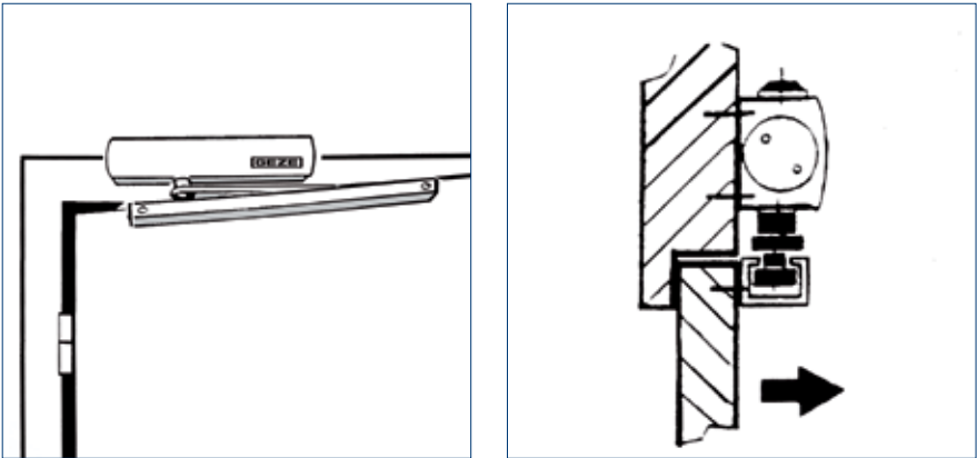
TS 5000 transom installation/hinge side
