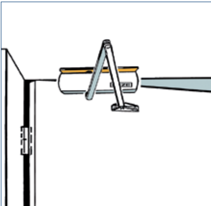
TS 2000 V transom installation/opposite hinge side lintel casing bracket
