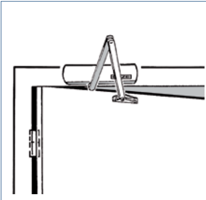
TS 2000 V transom installation/opposite hinge side
