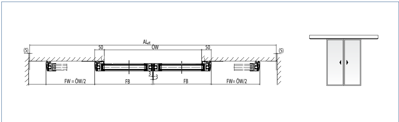
2-leaf, wall installation
