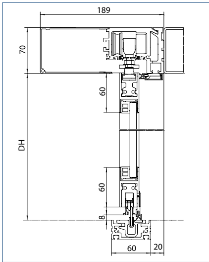
2-leaf door system
