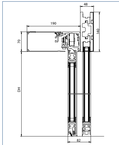
High girder section
