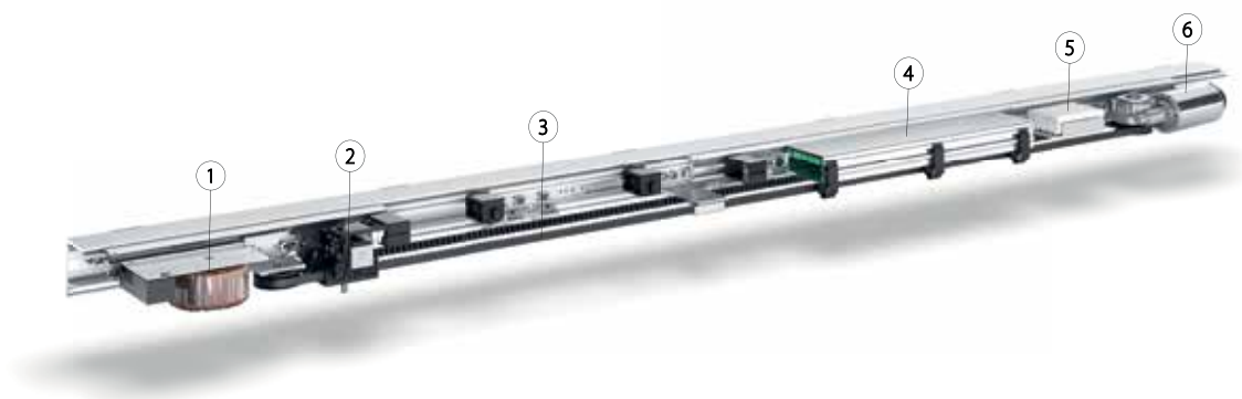
1 = Transformer | 2 = Locking mechanism | 3 = Roller carriage | 4 = Control unit | 5 = Rechargeable battery | 6 = Motor
