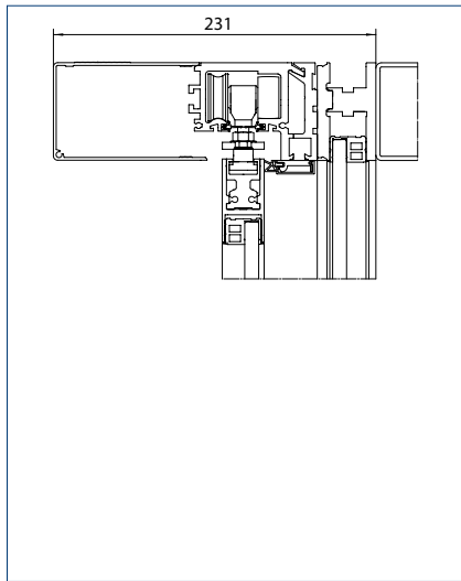
Drive with side panels on bolt profile
