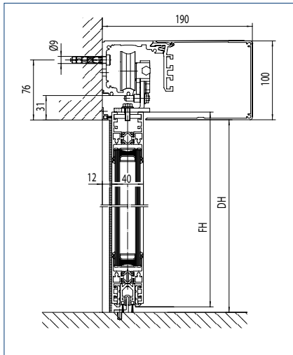
Wall installation, angled floor guide
