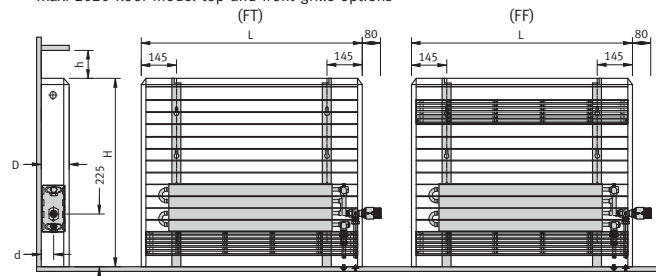
Maxi 2020 floor model top and front grille options (FT)
