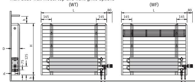
Maxi 2020 wall model top and front grille options (WT)
