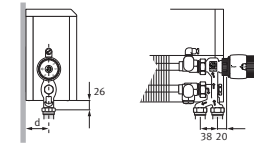
Example with Jaga Pro valve: to the wall or to the floor
