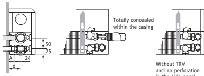
Example with Jaga valve: to the wall
