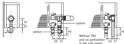
Example with Jaga valve: to the floor
