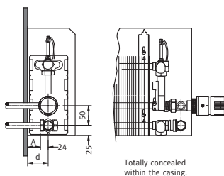
Example with Jaga valve: to the wall.
