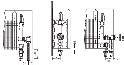
Example with Jaga Pro valve: to the floor - WT only.
