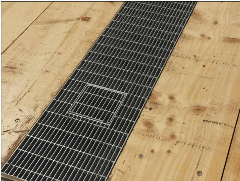
Walkways, Ventilation, Vehicular Type SP - 57x13/60x2SP/60x3mm (Galvanised)
