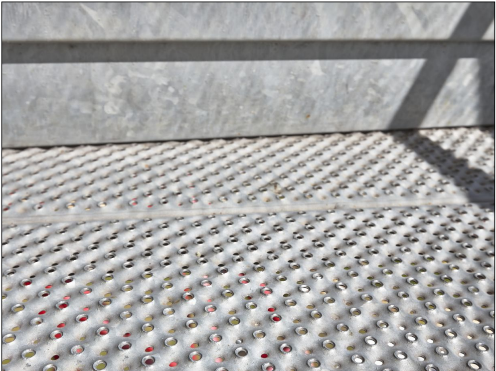
Walkways, Stair Treads/Landings Type O5-M - 215/45+15x2mm welded into shaped modules (Galvanised)
