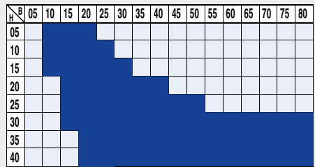
Unit sizes (10 ≙ 1 filter element)
