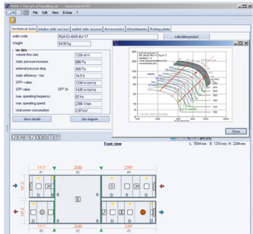
A configuration and design tool facilitates project design
