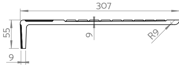
Fig 1. Side view of SN293/WL/307UR stair nosing.
