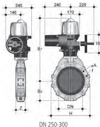
FK Butterfly Valve - Electrically actuated Disc
