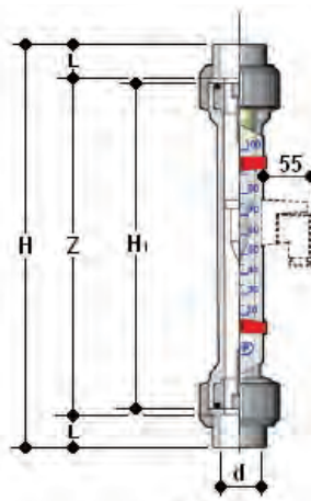
Variable Area Flowmeter with Metric series female ends
