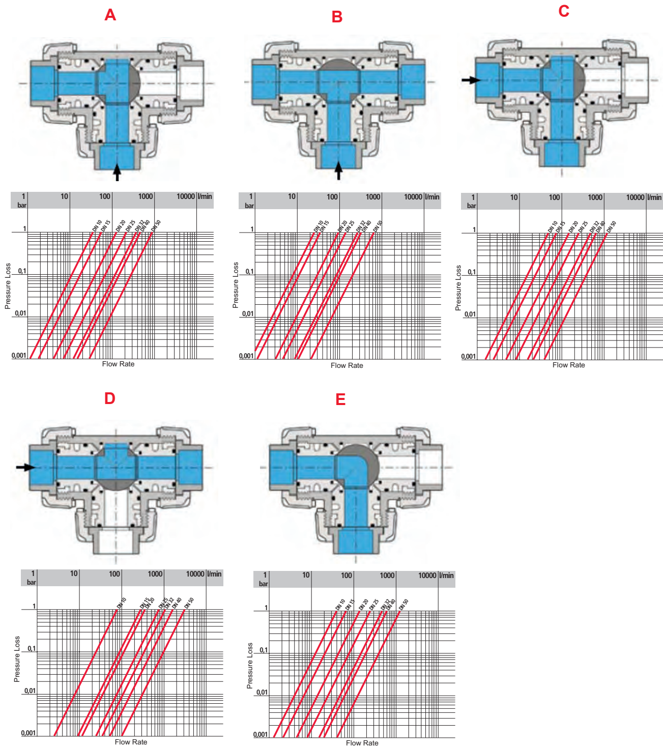
Pressure loss charts
