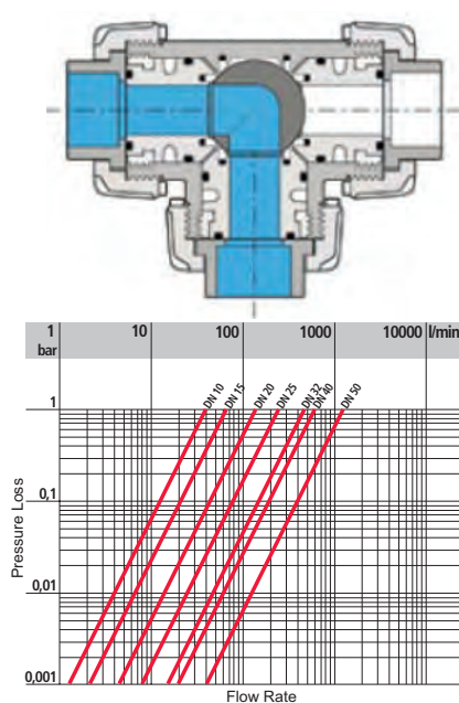
Pressure loss charts
