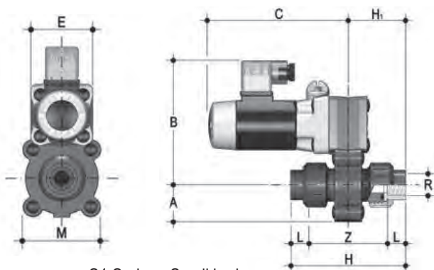
S1 Series - Small body
