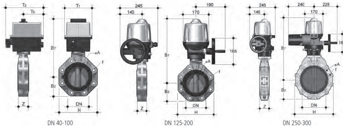
FK Butterfly valve - Electrically actuated Disc
