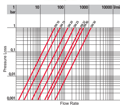
Pressure loss charts
