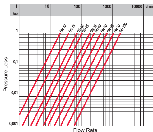
Pressure loss chart.
