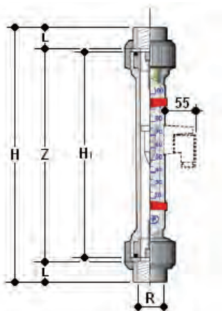
Variable Area Flowmeter with BSP series female ends, available in PVC-U.
