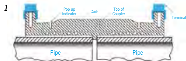
Pipe positioned in coupler prior to energising coil.
