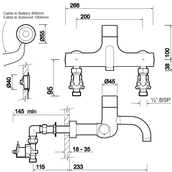
Detachable spout
