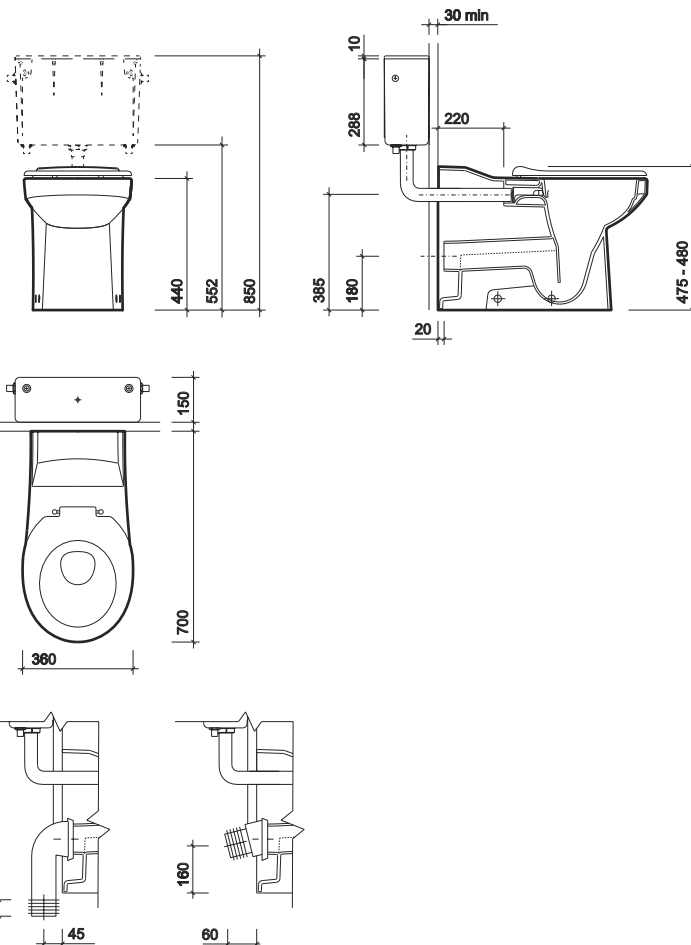
Avalon rimless 700mm projection back-to-wall WC pan
