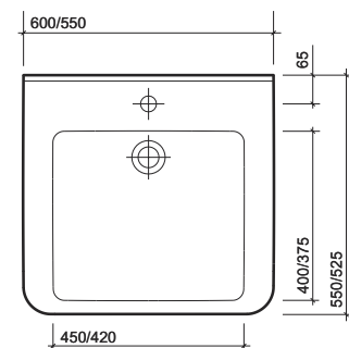
All 600 x 550mm basin
