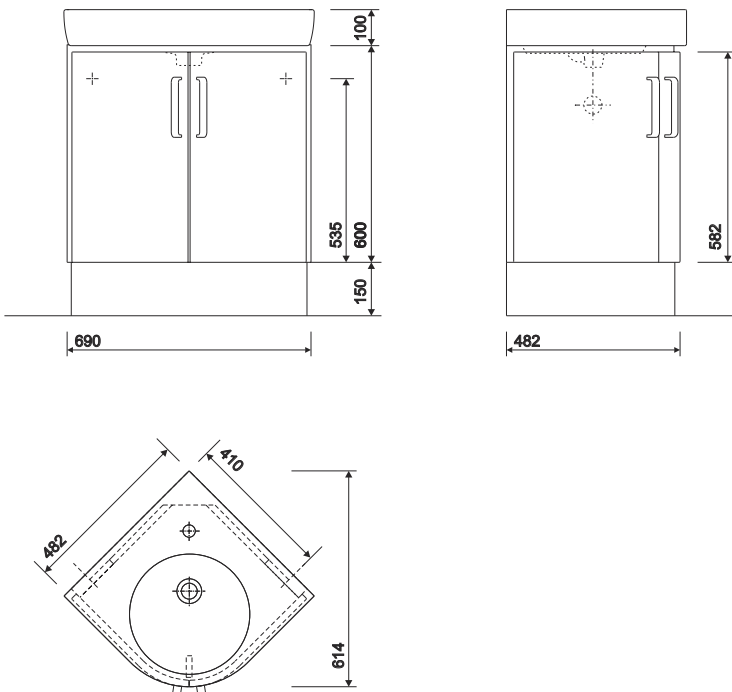
E200 500mm 1TH corner washbasin - grey furniture
