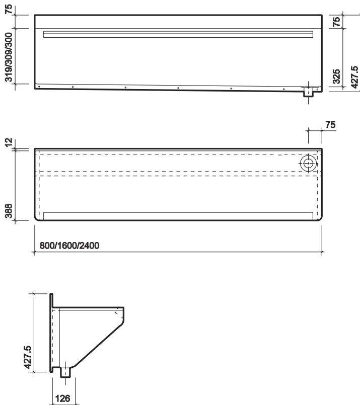
Scrub-up trough 800mm (RH outlet illustrated)
