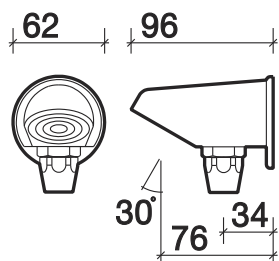
sola shower vandal resistant head
