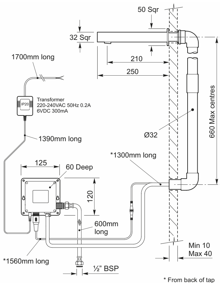
Sola wall mounted infra red spout, square
