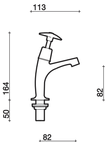
High neck cross head pillar taps
