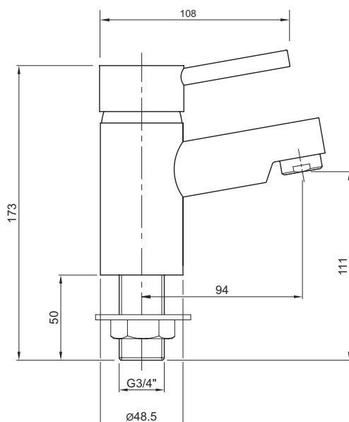
X60 Bath 3/4" Pillar Taps
