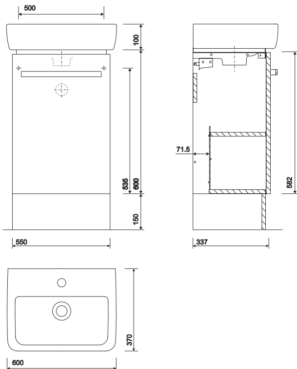
E200 600mm 1TH washbasin - white furniture
