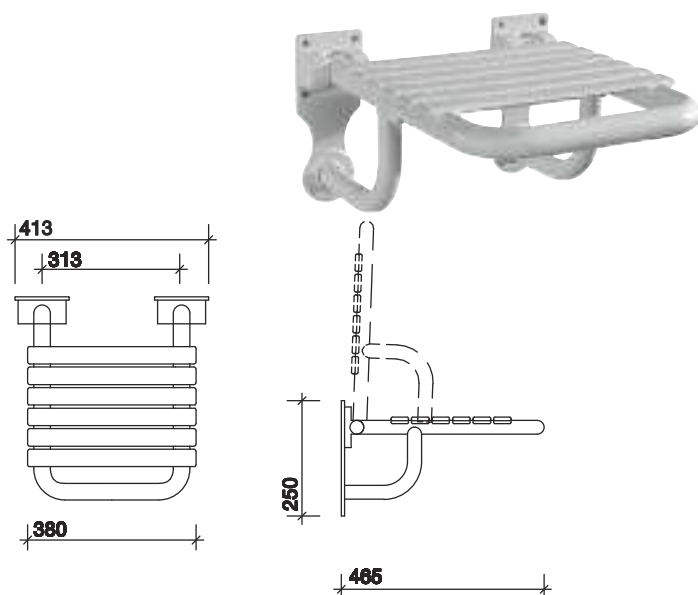
Shower seat
