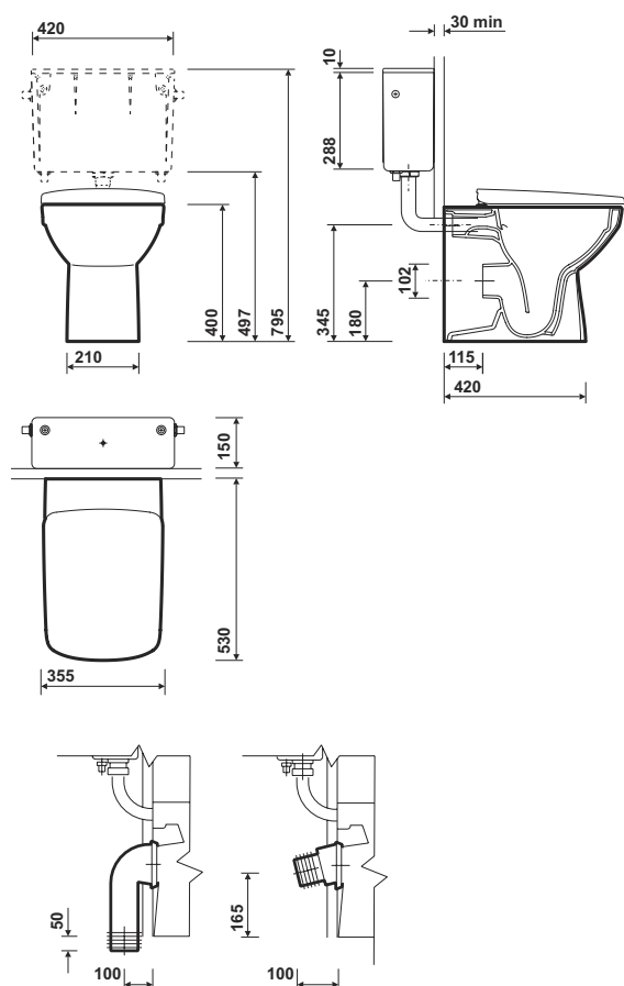
E100 rimfree ® square back-to-wall WC Suite, horizontal outlet
