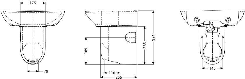
Semi pedestal for 450mm wash basin
