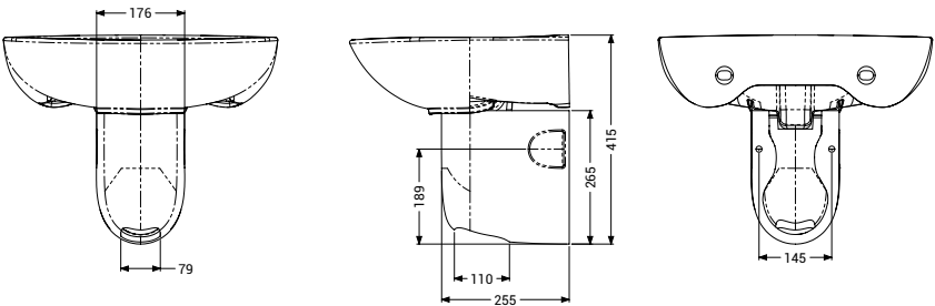
Semi pedestal for 550mm wash basin
