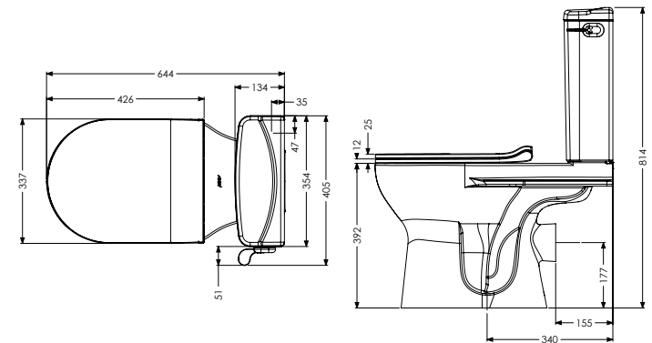
Livenza Plus close-coupled WC with lever flush
