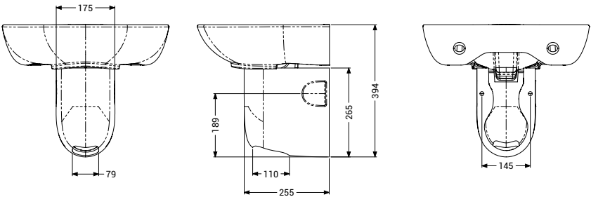
Semi pedestal for 500mm wash basin
