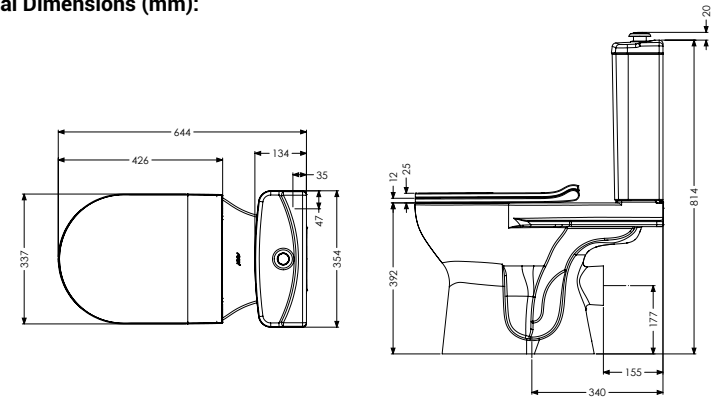
Livenza Plus close-coupled WC with raised push button flush
