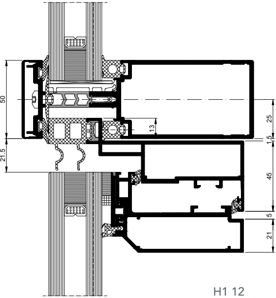
Cill Detail
