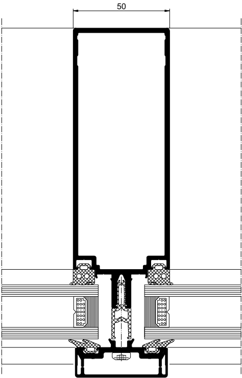
Intermediate Mullion
