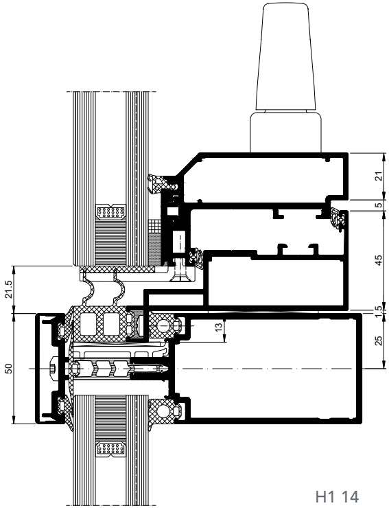
Cill Detail
