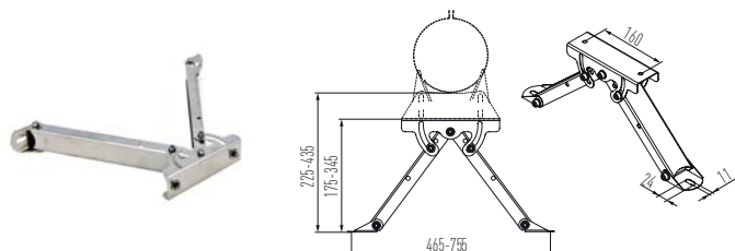
Wall Band Adjustable
