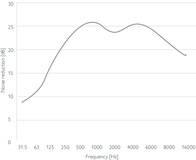
Average performance MFSIC1 100 - 600
