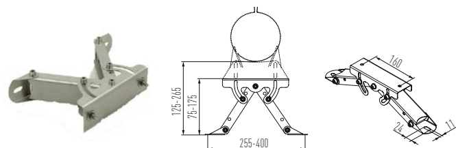
Distance Block for MFMB (Ø100 - 300)
