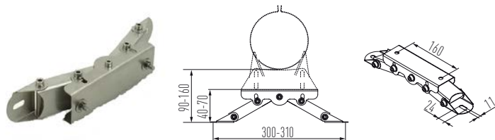
Distance Block for MFMB (Ø100 - 300)
