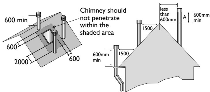
Fig. C BS 5440-1 Outlet siting for Gas Appliances (<70kW)
