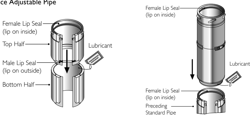
Fig. 3 2-Piece Adjustable Pipe
