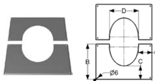
Roof plate 35°- 45° PMSA 25
