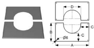
Roof plate 0°- 5° PMSA 25
