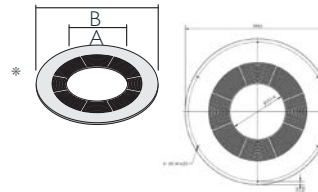
Round ventilated firestop
