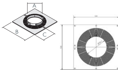
Ventilated support plate
