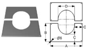
Roof plate 20°- 35° PMSA 25
