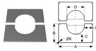
Roof plate 5°- 20° PMSA 25
