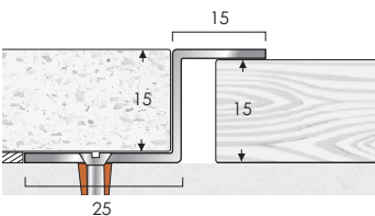
TIMBERLINE 2/22S Screw size 6
