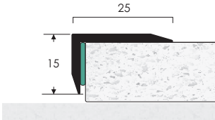
PTP 25/15 ISF
