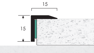
PTP 15/15 ISF
