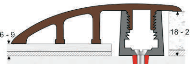
Kliks KSP73 Ramp Top with KB3 Base
