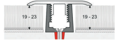
Kliks Twin Top with KB3 Base
