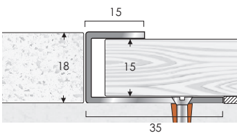
TIMBERLINE 1/22S Screw size 6
