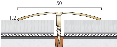
BC50 Screw size 6
