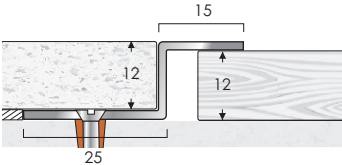
TIMBERLINE 2/15S Screw size 6
