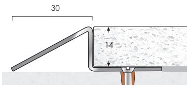
SR14 Screw size 6
