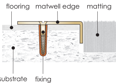
cross section view
