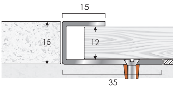
TIMBERLINE 1/15S Screw size 6
