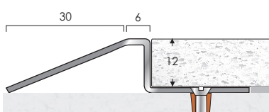
FTRS 12 Screw size 6
