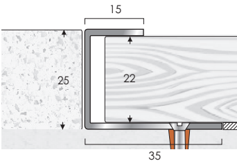
TIMBERLINE 2/12S Screw size 6
