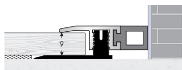
Kliks Slim End Stop with Expansion/Compression Feature with KKSBP12 uPVC Base Compatible with other bases
