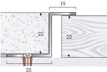
TIMBERLINE 2/22S Screw size 6
