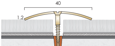
BC40 Screw size 6
