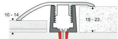
Kliks Ramp with KB3 Base
