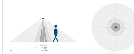
theLuxa S360 detection range and coverage.
