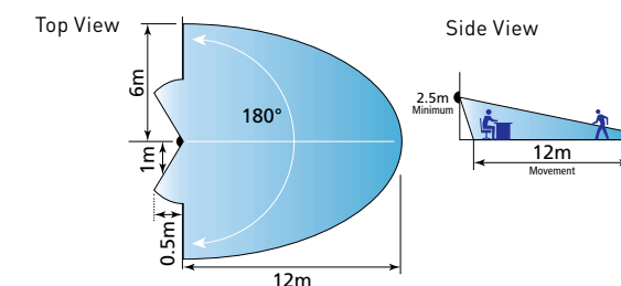
LED400PIR detection range and coverage.
