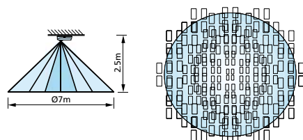
PDSM/PDFM detection range and coverage.
