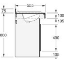
CV3 Profile Fully inset basin with upstand
