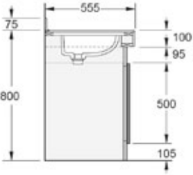
H3 Profile Fully inset basin with upstand
