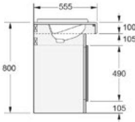
K4 Profile Fully inset basin without upstand
