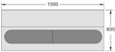
Lollipop Front Elevation shown K2 Profile only at 600mm high
