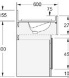
Baby Change Profile Fully inset basin with upstand
