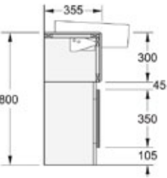
H2 Profile Semi-recessed basin without upstand
