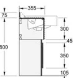
CV1 Profile Semi-recessed basin with upstand
