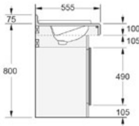
K3 Profile Fully inset basin with upstand
