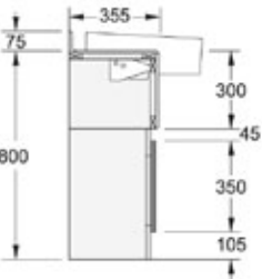
H1 Profile Semi-recessed basin with upstand
