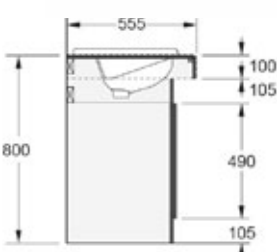
CV4 Profile Fully inset basin without upstand
