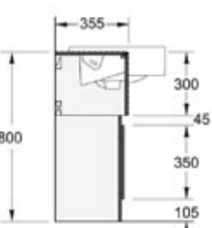
CV2 Profile Semi-recessed basin without upstand
