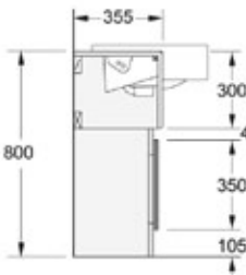
K2 Profile Semi-recessed basin without upstand
