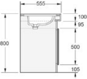
H4 Profile Fully inset basin without upstand
