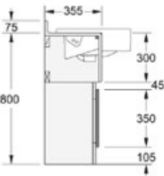
K1 Profile Semi-recessed basin with upstand
