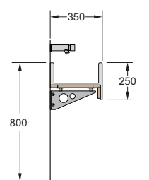
WT4 Profile Trough with wall mounted taps and cantilever brackets
