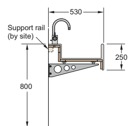
WT3 Profile Trough with deck mounted taps and cantilever brackets
