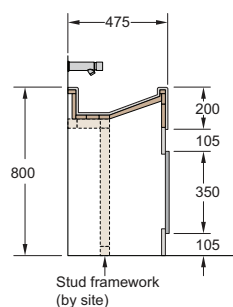
WT2 Profile Trough with wall mounted taps and underframe
