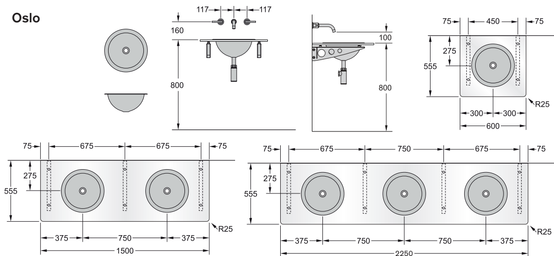
G4/Q4 Profile Fully inset basin without upstand
