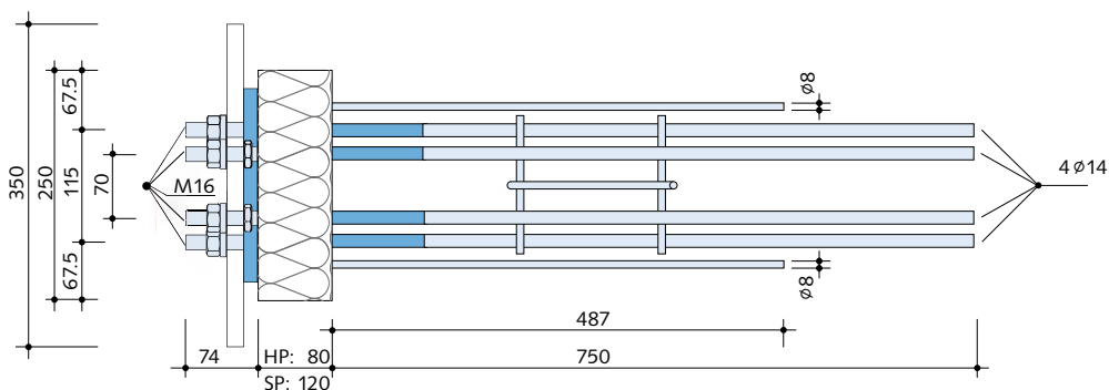
Plan view
