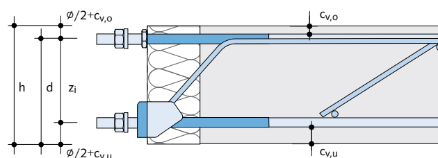
Inner cantilever and component height
