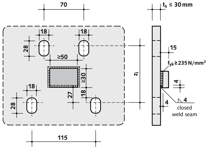
Hole layout for HIT-SDV and HIT-SMV with M16 thread (HIT-HP/SP SDV-2M16, HIT-HP/SP SMV-2M16)
