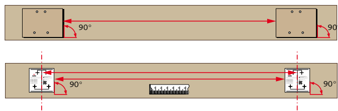
Figures: above: Installation aid on formwork using drill templates below: Installation aid on formwork – aligned
