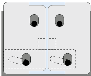
Figure A: Threaded bolt positioned at the bottom of the slot
