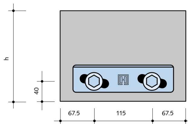
Figure: Spacings for HIT-SZV with M16 thread
