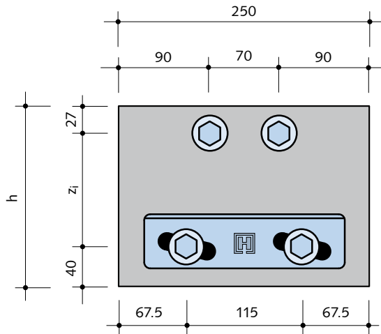
Spacings with HIT-SDV and HIT-SMV with M16 thread
