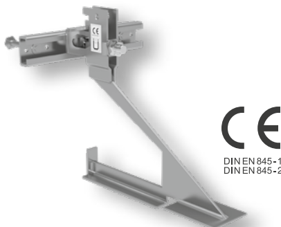
HALFEN HK5 Support bracket system for brickwork
