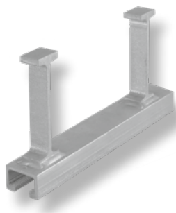
HALFEN HZA-PS Cast-in channel
