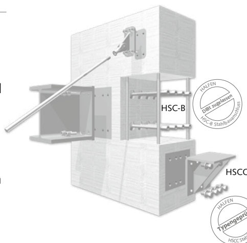
HALFEN HUC Universal Connection
