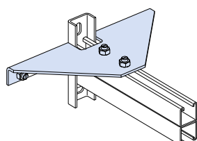
Assembly example with bracing KON Z1 (see page 31)
