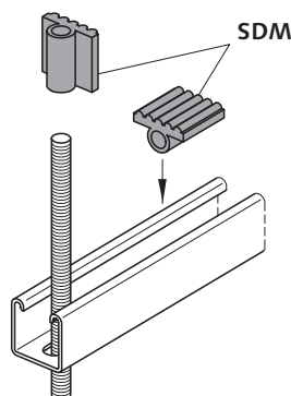
Assembly diagram
