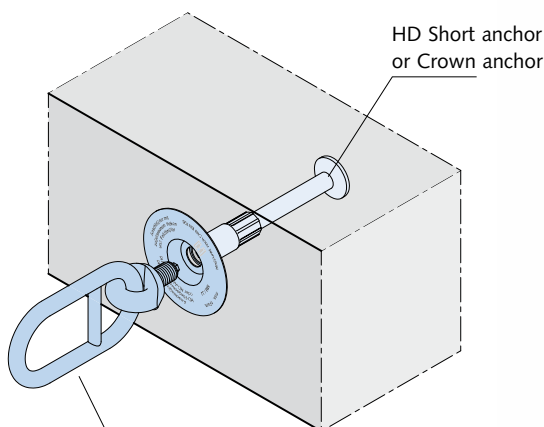
HD Link or ring bolt; is attached during installation as a permanent fixture.
