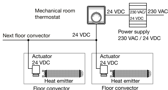
Room thermostat for connection of UN models with remote control
