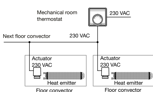
Room thermostat for connection of UN models with 230 VAC actuators
