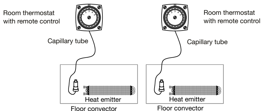
Room thermostat for connection of UN models with remote control
