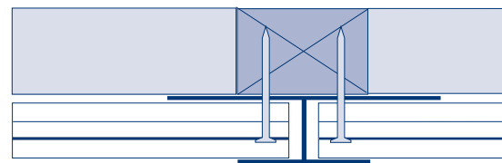
Fig. 20 Standard joint for long runs, using C033 cover trim
