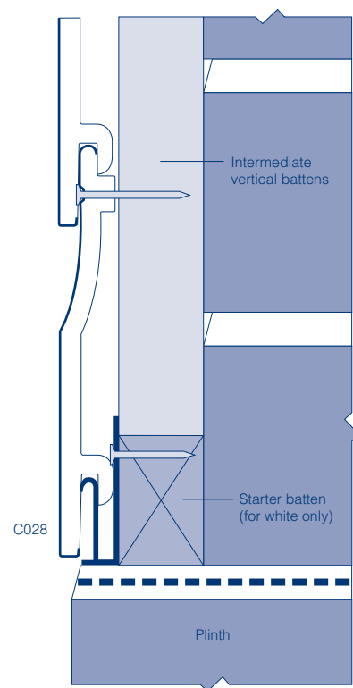
Fig. 8 Wall starter trim at solid base
