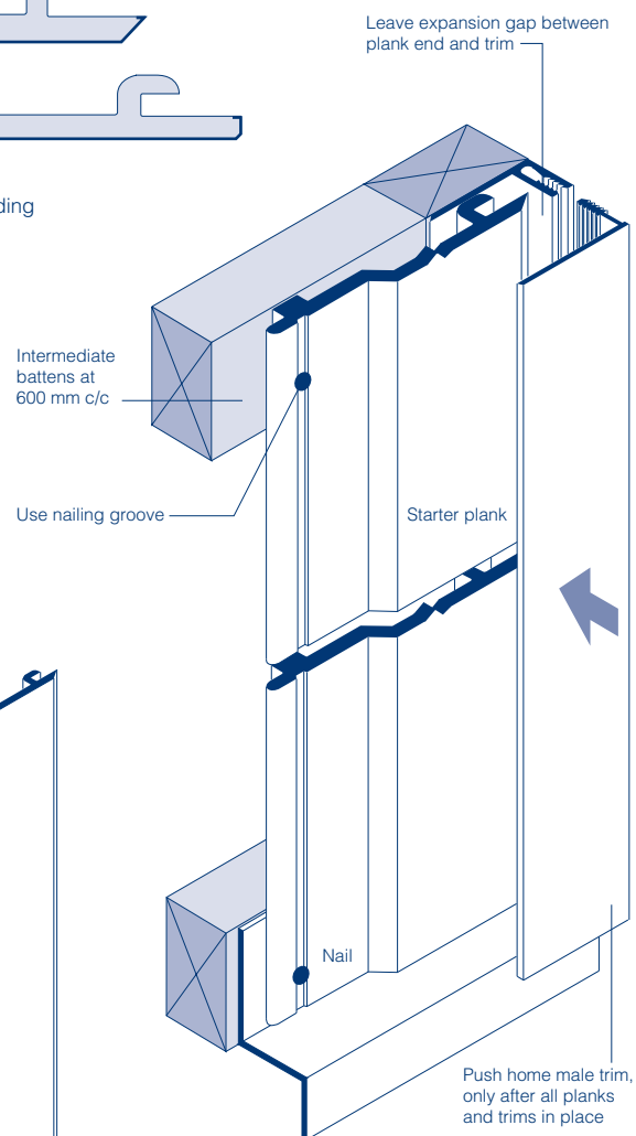
Fig.32 Locating starter plank (working right to left)
