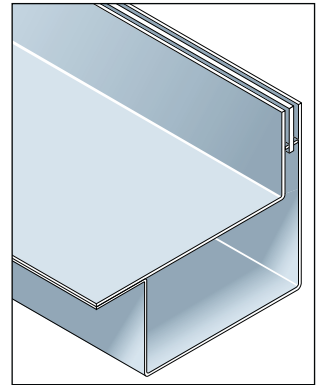
Spec. Code: HSCE Designed for use against a wall. With non-removable toe bar. 6mm slot width suitable for use in barefoot areas.
