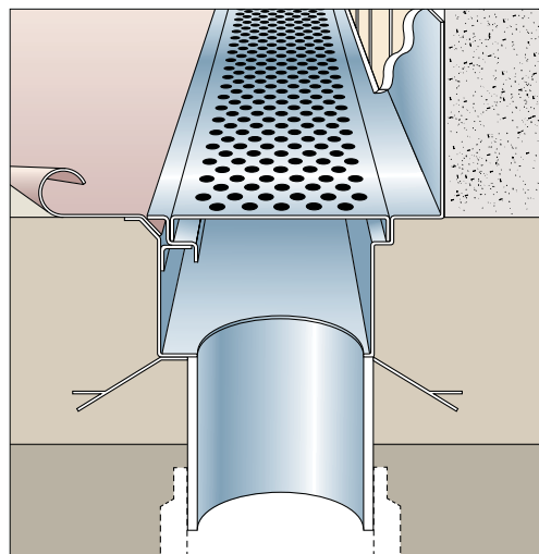
SVFT channel (SVF with optional tile upstand) and SS40135A1 grating.
