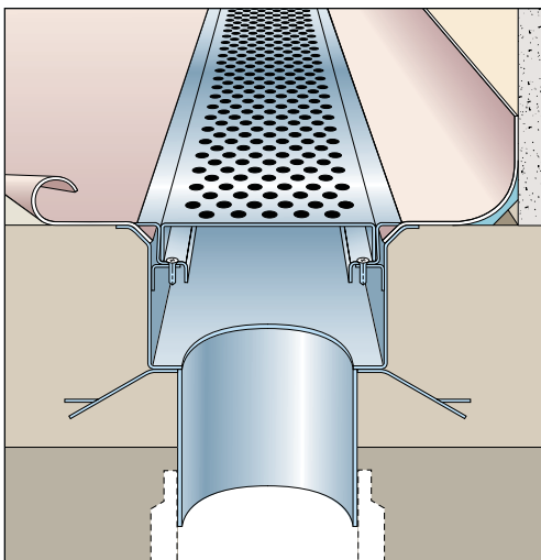
SVF channel and SS40135A1 grating, spaced away from wall, vinyl dressed both sides.
