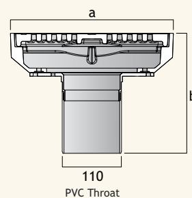
Bezel Connection Options for Square Heavy Duty Grate
