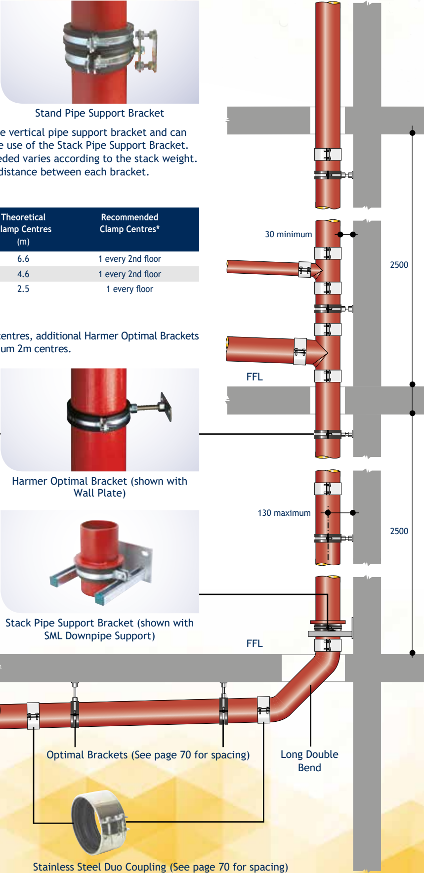
Stand Pipe Support Bracket Centres
