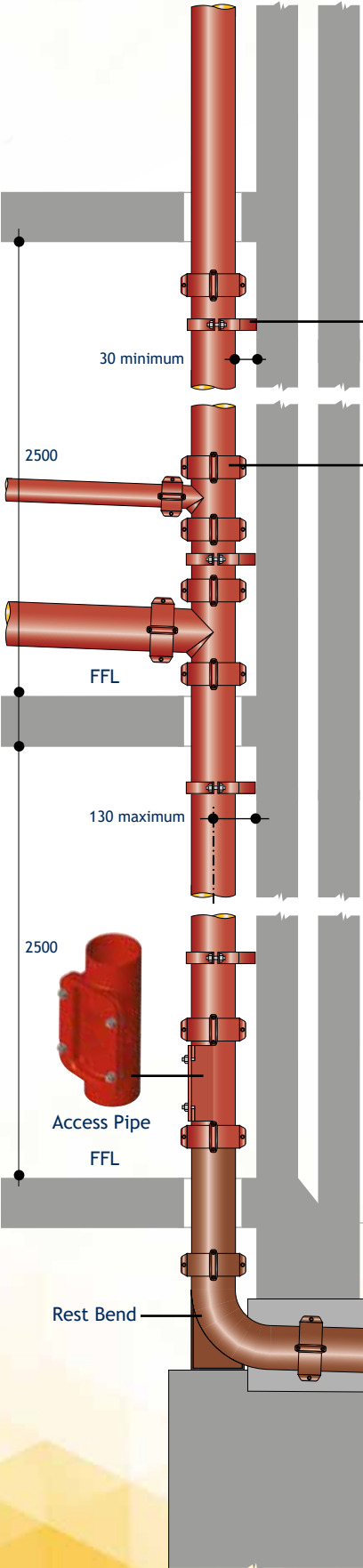
Stack Pipe Support Bracket Centres (when using Optimal Brackets)
