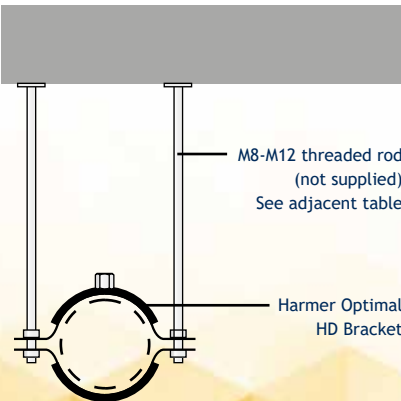
Alternative arrangement for pipework with drop length over 1 metre
