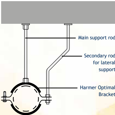
Harmer SML horizontal bracket and fixing arm
