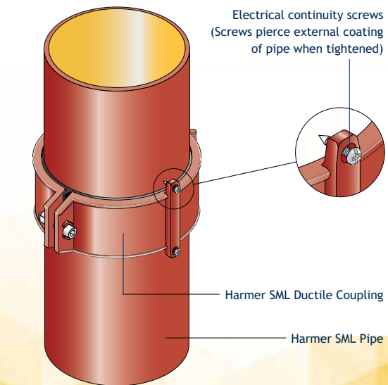
Harmer Ductile Coupling installation
