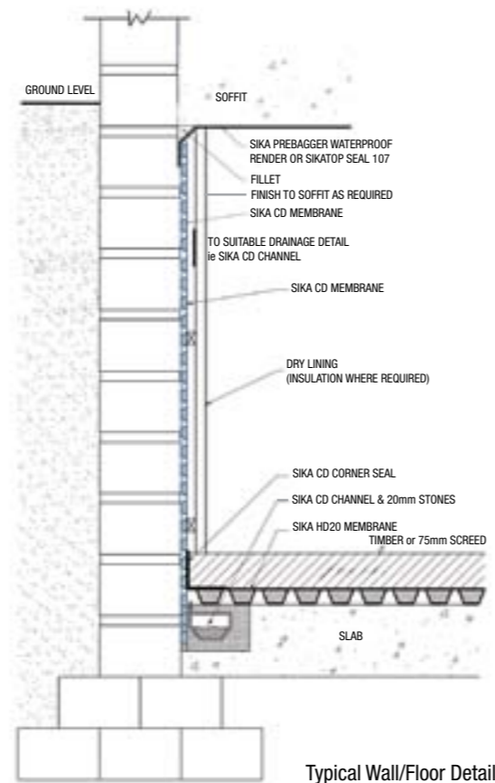
Typical Wall/Floor Detail
