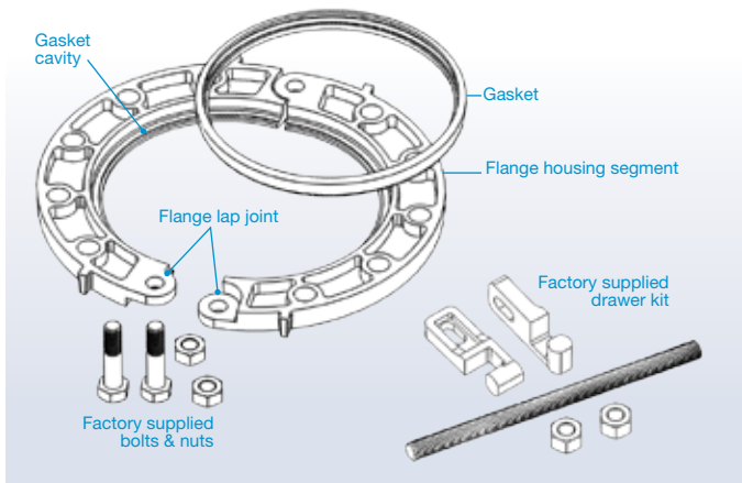
FLANGE ADAPTER (14-24")
