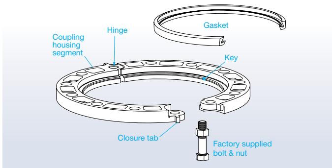
FLANGE ADAPTER (2-12")
