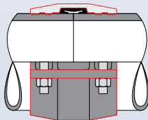
HDPE Pipe
