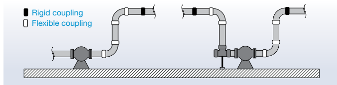
RIGID COUPLING, FLEXIBLE COUPLING
