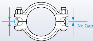
Metal-to-metal contact
