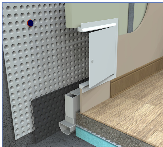
Figure 1: The Newton Basedrain channel captures water from the drainage membranes, and includes inspection ports for maintainability
