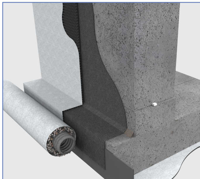
Figure 2: Newton 410 GeoDrain used externally to protect the waterproofing membrane as part of the Newton HydroBond System
