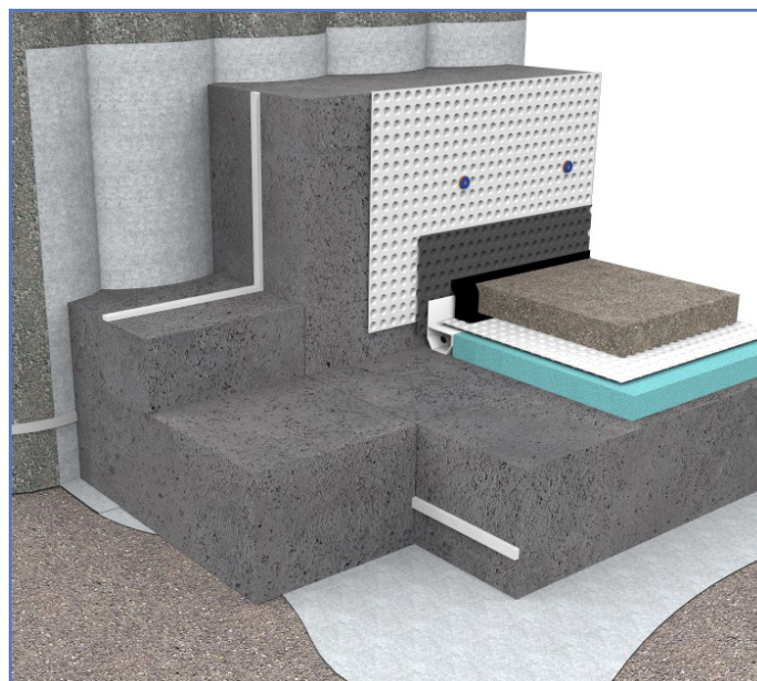
Figure 3: Comprehensive waterproofing with Type A protection externally, Type B protection integrally, and Type C protection internally
