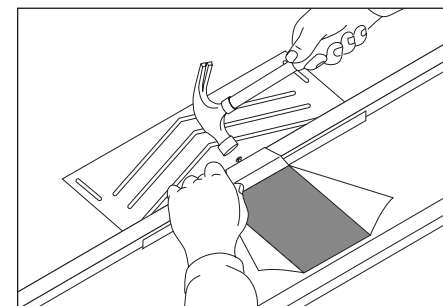
Fig. 5 – Secure soaker tray
