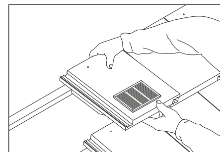
Fig. 6 – Fix contour tile vent
