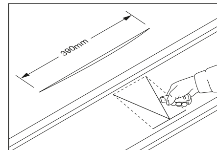
Fig. 4 – Make aperture in underlay
