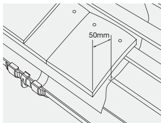
Fig. 11 – Ensure sufficient overhang into gutter
