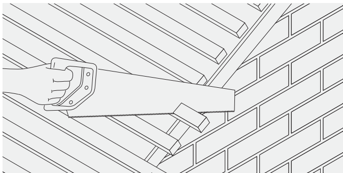
Fig. 49 – Saw battens flush
