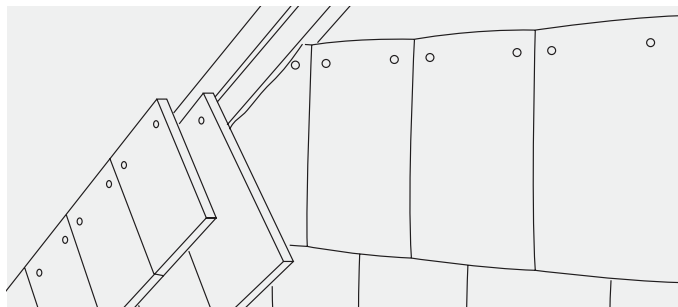
Fig. 32 – Fixing double soldier course of tiles to raked batten
