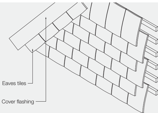
Fig. 31 – Cut tile to meet rake of verge
