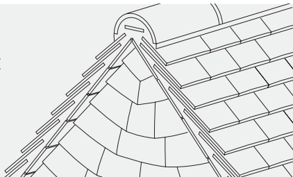
Fig. 29 – Cut tile-and-a-half tile
