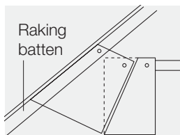
Fig. 30– Apex of gable
