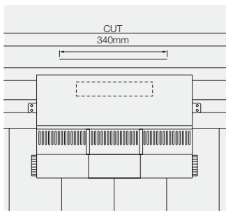
Fig. 87 – Position and fix in-line vent unit
