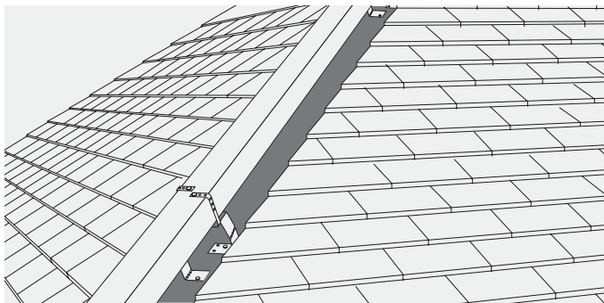
Fig. 57 – Fixing hip batten
