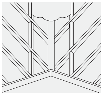
Fig. 68 – Use of support noggins
