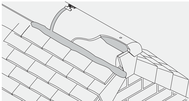
Fig. 53 – Mortar bedded stop end ridge tile used to finish cloak verge at ridge
