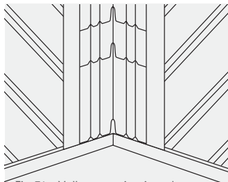
Fig 71 – Valleys terminating above eaves level
