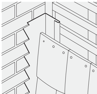
Fig. 35 – Abutment to wall, with flashing
