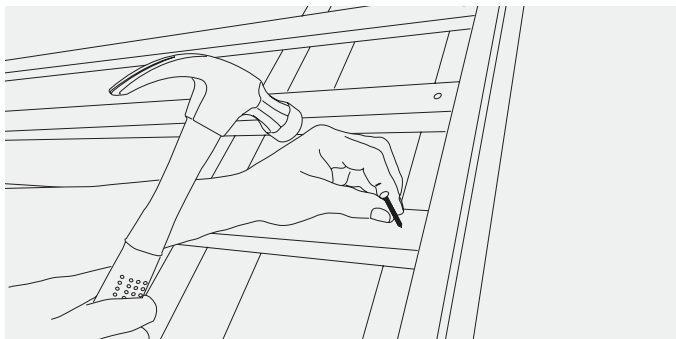
Fig. 47 – Nailing verge units
