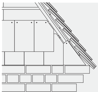
Fig. 33 – Cut tile to meet rake of verge
