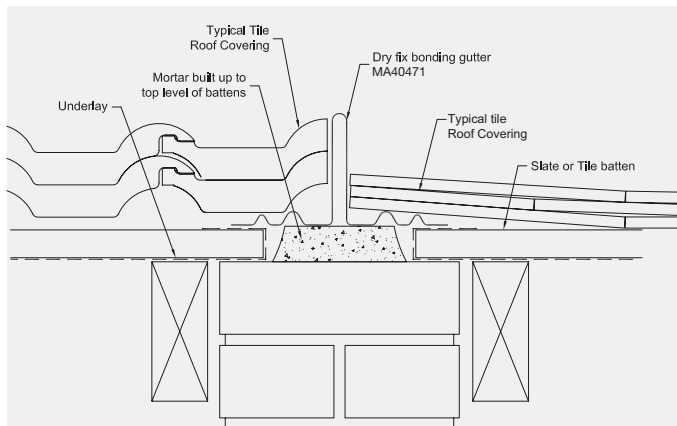
Fig. 91 – Typical firebreak installation showing high profiled interlocking tiles abutting slates, using MA40471
