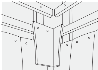
Fig. 26 – Internal angle with Internal Angle tiles
