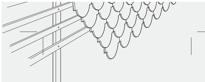
Fig. 25 – Feature tiles laid over battens and counter battens
