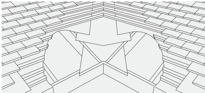
Fig. 18 – Laying valley tiles
