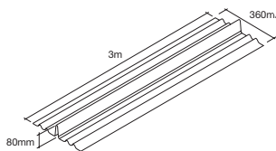
Low profile GRP valley (30422)
