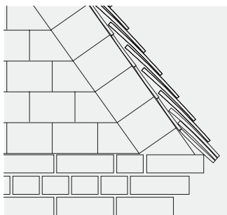
Fig. 34 – Fixing tiles to raked batten
