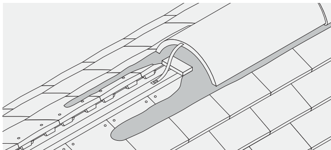
Fig. 20 – Typical bedded ridge with traditional galvanised security wire
