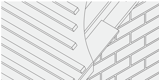
Fig. 50 – Fibre cement strip inserted under battens, 50mm overhang
