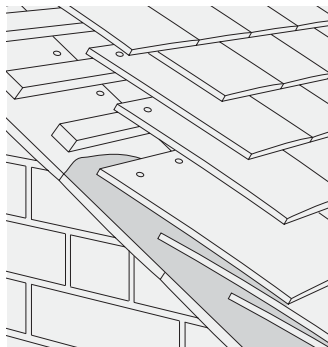
Fig. 14 – Undercloak using Plain tiles
