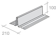
High profile bonding gutter (code MA40471)
