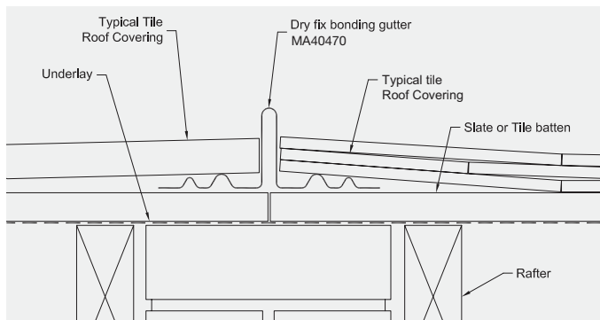
Fig. 89 – Typical standard installation showing low profiled interlocking tiles abutting slates, using MA40470
