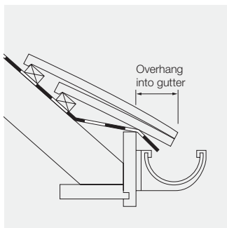
Fig. 7 – Measuring gutter overhang
