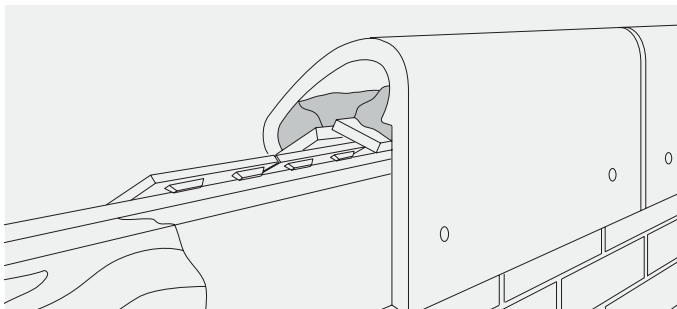
Fig. 22 – Bedded mono-ridge with 2 mechanical fixings
