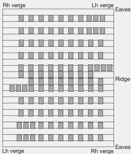
Fig. 1 – Loading roof evenly with tile/slate stacks
