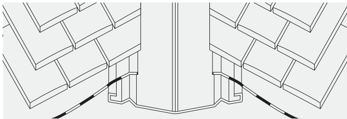
Fig. 19 – Metal valley construction for plain tiles
