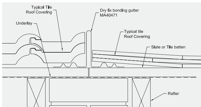
Fig. 90 – Typical standard installation showing high profiled interlocking tiles abutting slates, using MA40471
