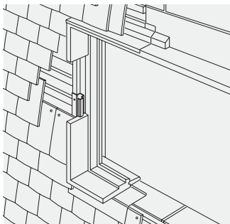
Fig. 36 – Abutment to window
