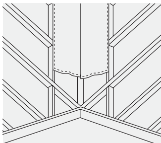
Fig. 67 – Butt joint valley boards over supporting rafters
