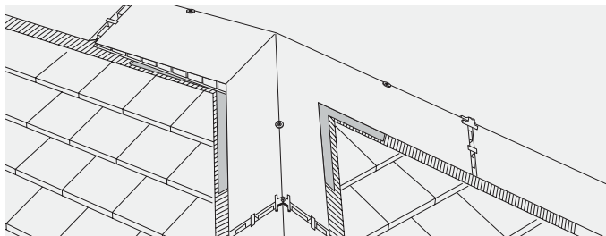
Fig. 65 – Weathering of hip/ridge junction with soaker
