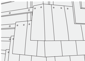
Fig. 27 – External angle with External Angle tiles
