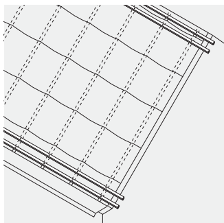
Fig. 6 – Setting out eaves/top course battens
