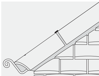
Fig. 16 – Bedded and mechanically fixed third round third hip ridge tiles used as hip capping with hip iron
