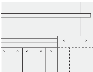
Fig. 12 – Setting out eaves with eaves course
