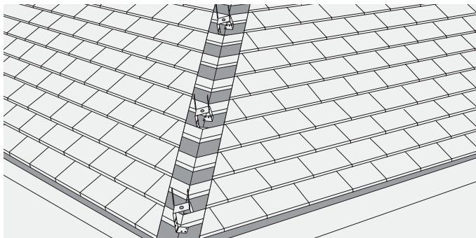
Fig. 56 – Lay tile to hip with raking cut
