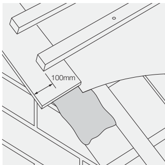
Fig. 15 – Undercloak using fibre cement strip
