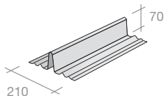
Low profile bonding gutter (code MA40470)
