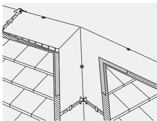
Fig. 64 – Weathering of hip/ridge junction with lead soaker
