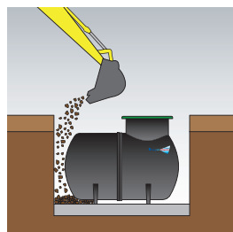
BACKFILL AND LEVEL
