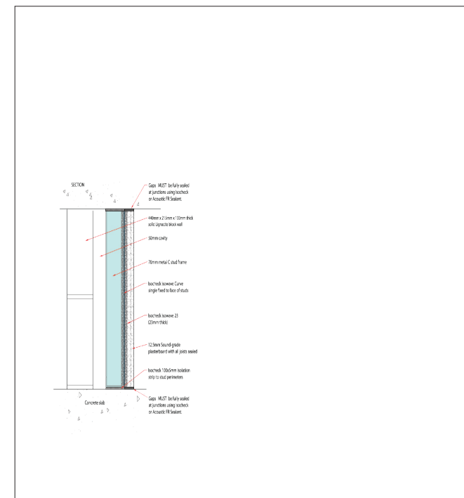
100mm Lignacite solid blockwork with acoustic lining to one side. Sound insulation = 64 R w , dB
