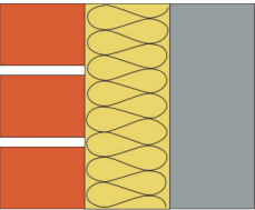
Full Cavity Fill and 100mm Lignacite blocks
