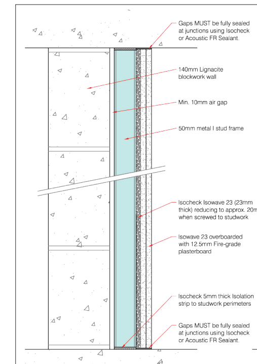
140mm Lignacite SP blockwork with acoustic lining to one side. Sound insulation = 56 R w , dB
