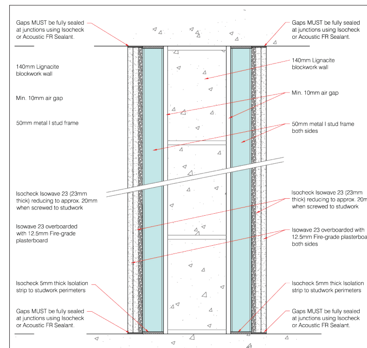
140mm Lignacite SP blockwork with acoustic lining to both sides. Sound insulation = 65 R w , dB
