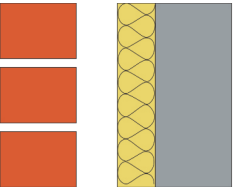
Partial Cavity Fill and 100mm Lignacite blocks
