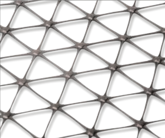
SC Intergrid. Proven structural performance with lower construction cost
