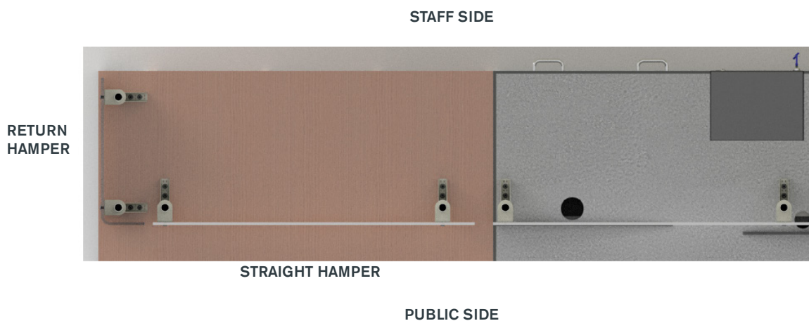
EXAMPLE STANDARD COUNTER LAYOUT - PLAN VIEW
