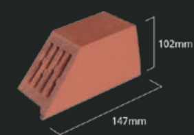
Unit TB 10 angled verge Tilebrick™
