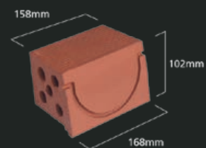
Unit TB 16 club Tilebrick™
