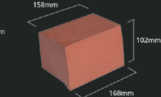
Unit TB 3 fair end 1 Tilebrick™
