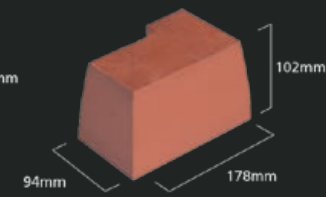
Unit TB 5 90° return 1x1/2 Tilebrick™
