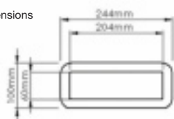
Duct Dimensions
