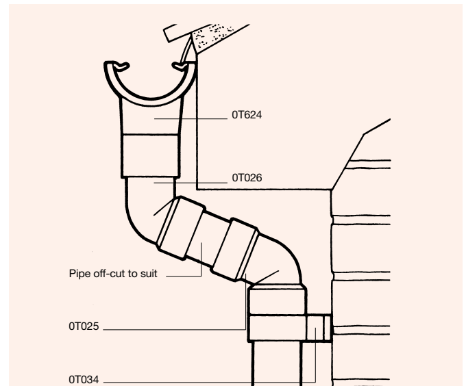
Figure 47: Offset on deep fascia
