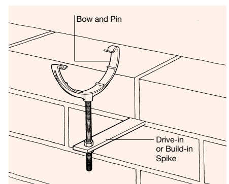
Figure 33: Rise and Fall Bracket Assembly
