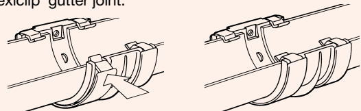
'Flexiclip' gutter joint.
