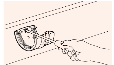
Figure 27: Installation of RoundLine Gutter Union
