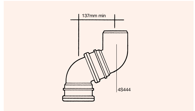
Figure 46: RoofLine shallow offset
