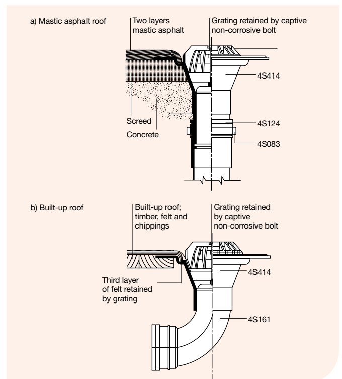
Figure 19: Roof Outlet installation
