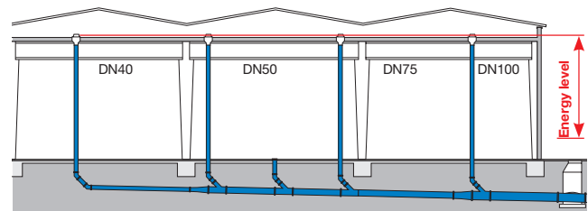
Figure 4: System components of the Wavin QuickStream system
