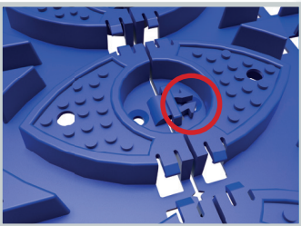
"SNAP CLIPS" to fasten the panels together.
