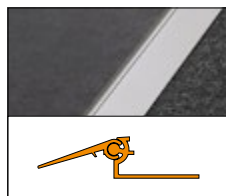
Schlüter®-RENO-V
