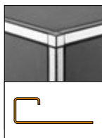
Schlüter®-QUADEC
