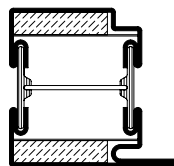
Janisol 2 EI30 RS/Smoke
