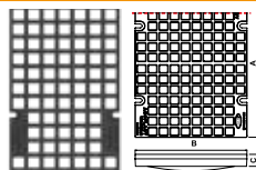
Ductile iron mesh grating
