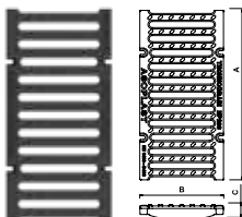
Ductile iron grating (18mm slot)
