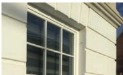
Type SDC water evacuation is in place with the discreet outlets set back in the rendered reveal.
