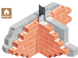
Vertical DPC for introduction into existing masonry skins
