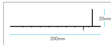
Leaving the insulation projecting the reveal and cutting it vertically afterwards is an alternative approach.
