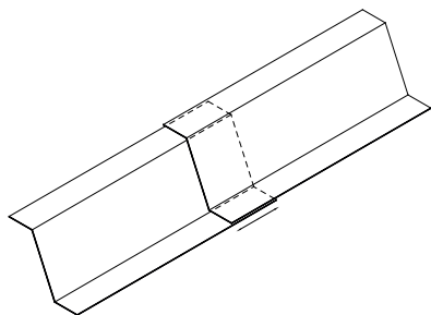
Lapping method of joining shown before application of sealing tape.
