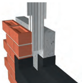
(Notching the closer face permits it to continue downwardly below the Type LTT level, so it terminates below opening level in the usual manner).
