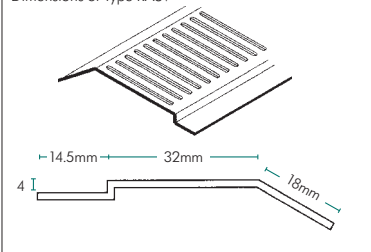
Dimensions of Type RASV
