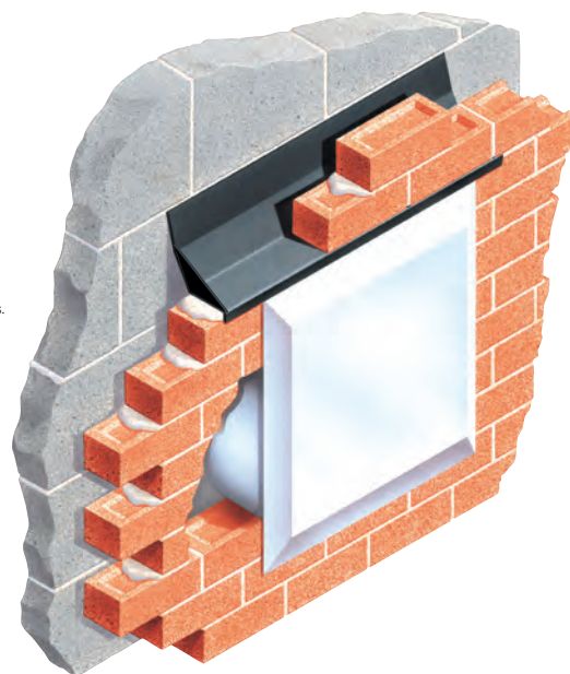
Type M Cavitray for use over meter boxes.
