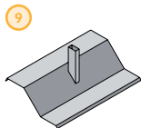
9 Type C/P with pipe projecting through cloak
