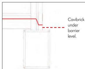
Membrane level will vary depending flooring construction. Barrier profile interfaces with membrane - inboard section shaped to suit membrane level / floor construction configuration.
