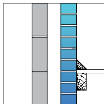
Rain penetrates the external skin, which becomes an internal skin below the new roofline.
