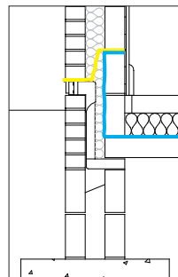
The design detail and the resultant as-built detail, demonstrating the necessity to rely on support from a convenient inner skin course can result in the arrangement being rather cumbersome.
